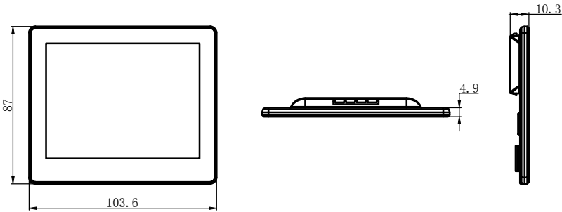
TECHNICAL DRAWINGS (mm)
